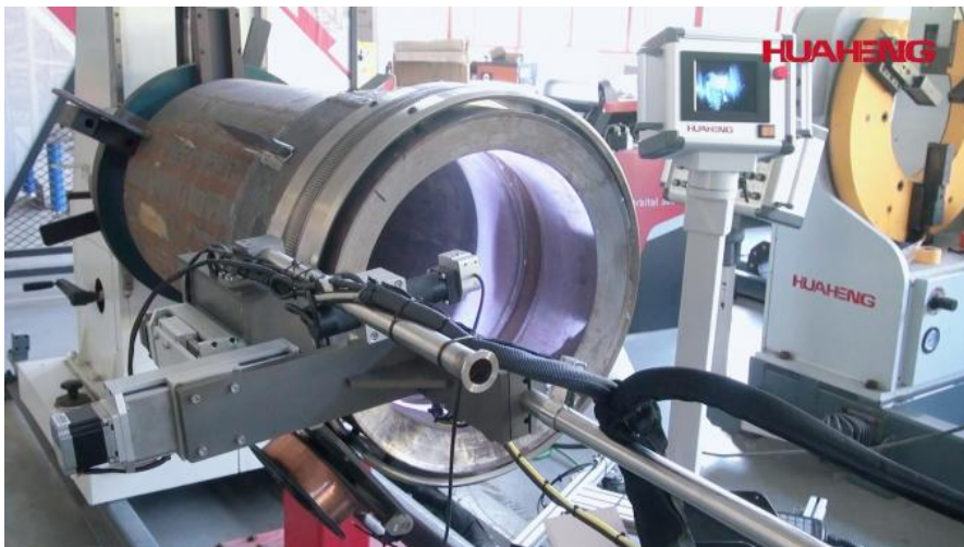
MIG TRACK 60 Welding Trolley System:
