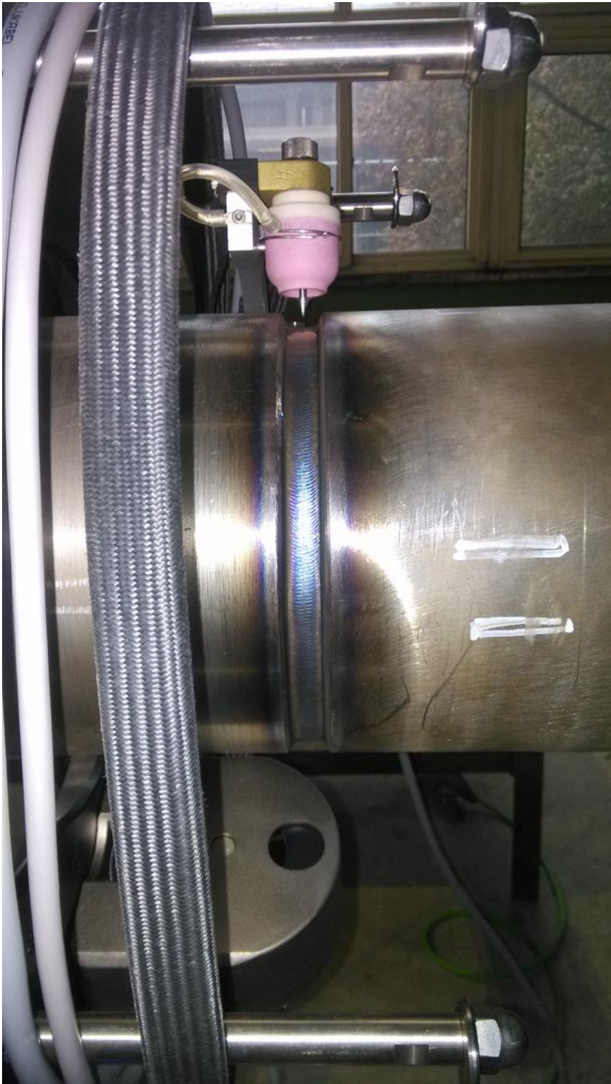
TOA40 Narrow Spacing Pipe Welding System:
